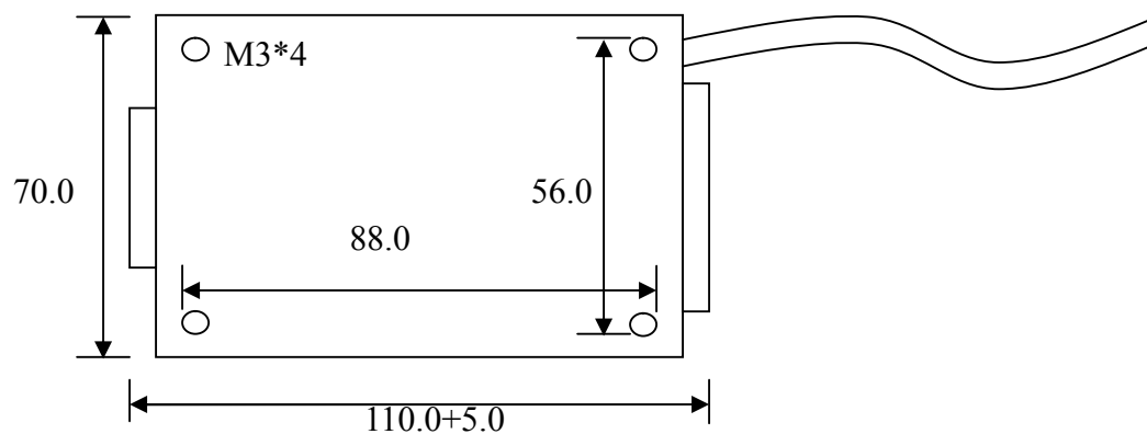
Dimension: (mm)
